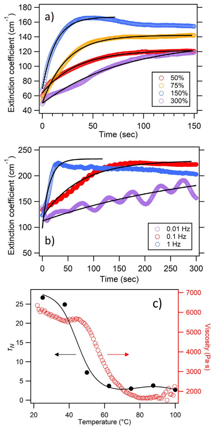
Figure 3. Time evolution of the extinction coefficient at the stopband wavelength of \lambda = 610 nm at a temperature of 50 ^{\circ}\text{C} . This is shown for various shear amplitudes at frequency 1 Hz in (a), and for various oscillation frequencies at a shear amplitude of 150\% in (b), as indicated. Exponential trend lines are used to extract shear-ordering timescales, as limited to the illustrated range of fitting. (c) Shows the temperature dependence of experimentally derived \tau_N values for parameters of frequency = 1 Hz and strain = 100\% , in comparison to the rheometrically measured viscosity. An indicative trendline is added to the former, using smoothing spline fitting.
