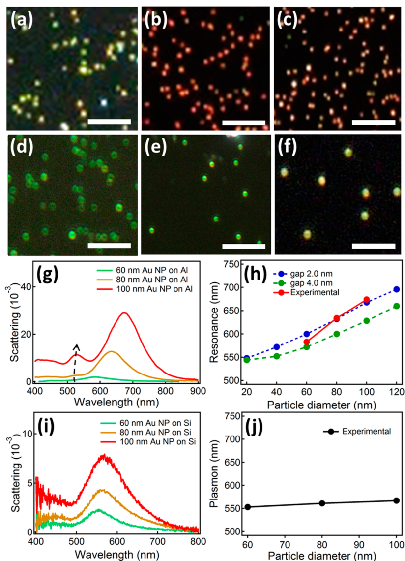
Figure 1. Dark field images of different sized Au NPs on Al mirror (a–c) and Si wafer (d–f). (a, d) 60 nm, (b, e) 80 nm, (c, f) 100 nm. Scale bars are 10 \mu\text{m} . (g, i) Scattering spectra of different sized Au NPs on (g) Al films and (i) Si wafers, with peak positions extracted in panels (h) and (j). The blue and green dashed lines in panel h are the simulated resonance positions for gap sizes of 2 and 4 nm \text{Al}_2\text{O}_3 .
