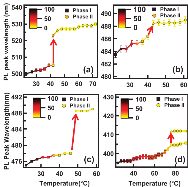
FIG. 4. Temperature dependence of PL maxima for C12PbI_{4(1-y)}Br_{4y} thin films of (a) y = 0.0 , (b) y = 0.37 , (c) y = 0.62 , and (d) y = 1.0 . (The color scale shows the relative PL intensity in arbitrary units).
