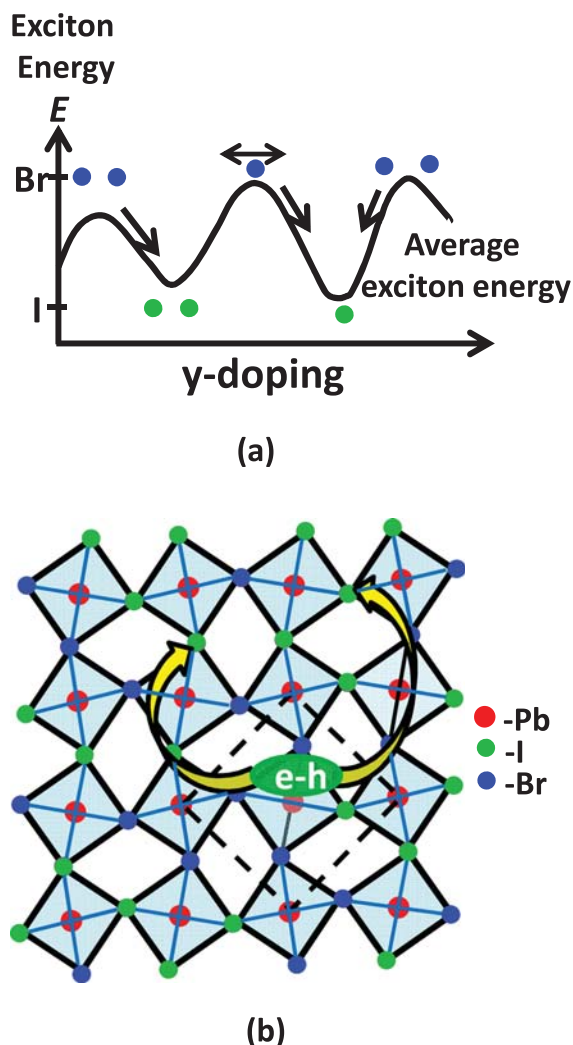
FIG. 6. (a) Schematic of exciton energy levels and the non-linear diffusion of excitons in mixed IO hybrids. (b) Schematic of Pb-I-Pb-Br network (top view) showing the diffusion of excitons from relatively high energy Pb-Br sites to lower energy Pb-I sites.
