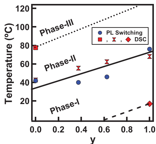
FIG. 8. Variation of phase transition temperatures obtained from PL peak switching studies and DSC (heating run) and with different y -value of C12PbI 4(1-y) Br 4y . The lines are guide to the eye, the dotted line (...) indicates T_2 , the solid line indicates T_1 and the dashed line (- - -) indicates T_0 transition temperatures.
