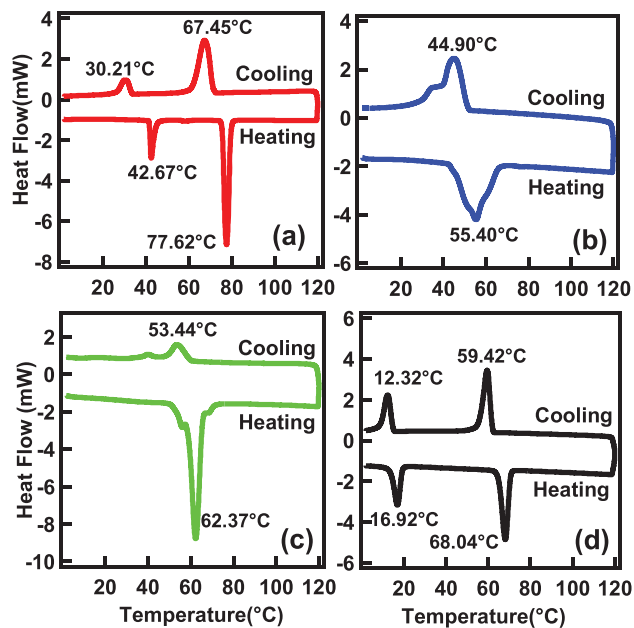
FIG. 5. DSC curves for powder samples of C12PbI_{4(1-y)}Br_{4y} at (a) y = 0.0 , (b) y = 0.37 , (c) y = 0.62 and (d) y = 1.0 . The cooling and heating scans are between 0 °C and 120 °C ( 5^\circ Cmin^{-1} ).
