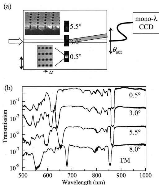
FIG. 1. (a) Design of planar PC waveguide chips containing several rectangular PC regions ( 500 \mu\text{m} \times 186 \mu\text{m} ), together with chromatic refraction detection geometry. Insets show scanning electron micrographs of the rectangular lattice in plan and cross section. (b) Normalized TM-polarized transmission spectra of four devices with a direction successively rotated away from the propagation direction by 0.5^\circ – 8^\circ , on a log scale and shifted vertically for clarity.
