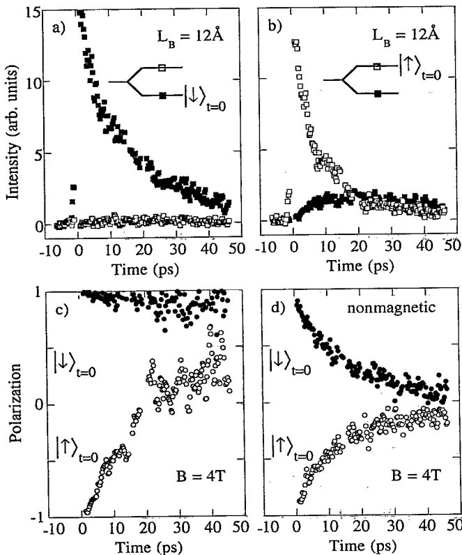
FIG. 2. Time- and spin-resolved PL from the sample of Fig. 1 at T=4.6 K in B=4 T for (a) carriers initially orientated spin-down, and (b) spin-up excited at 2.530 eV. In each case solid (open) symbols represent the energetically (un)favored spin-down (spin-up) component of the luminescence detected at 2.525 eV. (c) The resulting time-dependent polarization P = [I_{\downarrow} - I_{\uparrow}] / [I_{\downarrow} + I_{\uparrow}] , where solid (open) symbols represent the polarization from spin-down (spin-up) injected carriers. (d) Analogous measurements to (c) for a nonmagnetic control sample under similar conditions.
