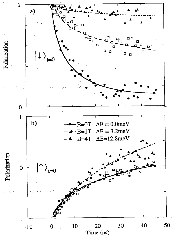
FIG. 3. Time-resolved polarization from the sample of Fig. 1 at T=4.6 K, excited 5 meV above the peak luminescence in increasing magnetic fields for carriers injected (a) spin-down, and (b) spin-up. Points have been removed for clarity and the lines serve as guides to the eye. The measured Zeeman splitting \Delta E is given for each field.
