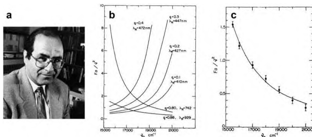
Fig. 6 (a) Photograph of Martin Moskovits. (b) The dependence of the quantity F_d/V^2 on exciting frequency v_0 for various values of \lambda_R , which is the resonance wavelength. The Raman intensity is proportional to F_d/V^2 . q is the volume fraction of the metal within a dielectric of dielectric constant \epsilon_0 . The quantity plotted is actually 6.69 \times 10^7 F_d/V^2 . (c) The solid line is the one of \lambda_R = 929 \text{ nm} in (b). Points are taken from ref. 72 and refer to the 1008 cm -1 ring vibration of pyridine. Reproduced from ref. 4 with permission. Copyright 1978 AIP publishing.
